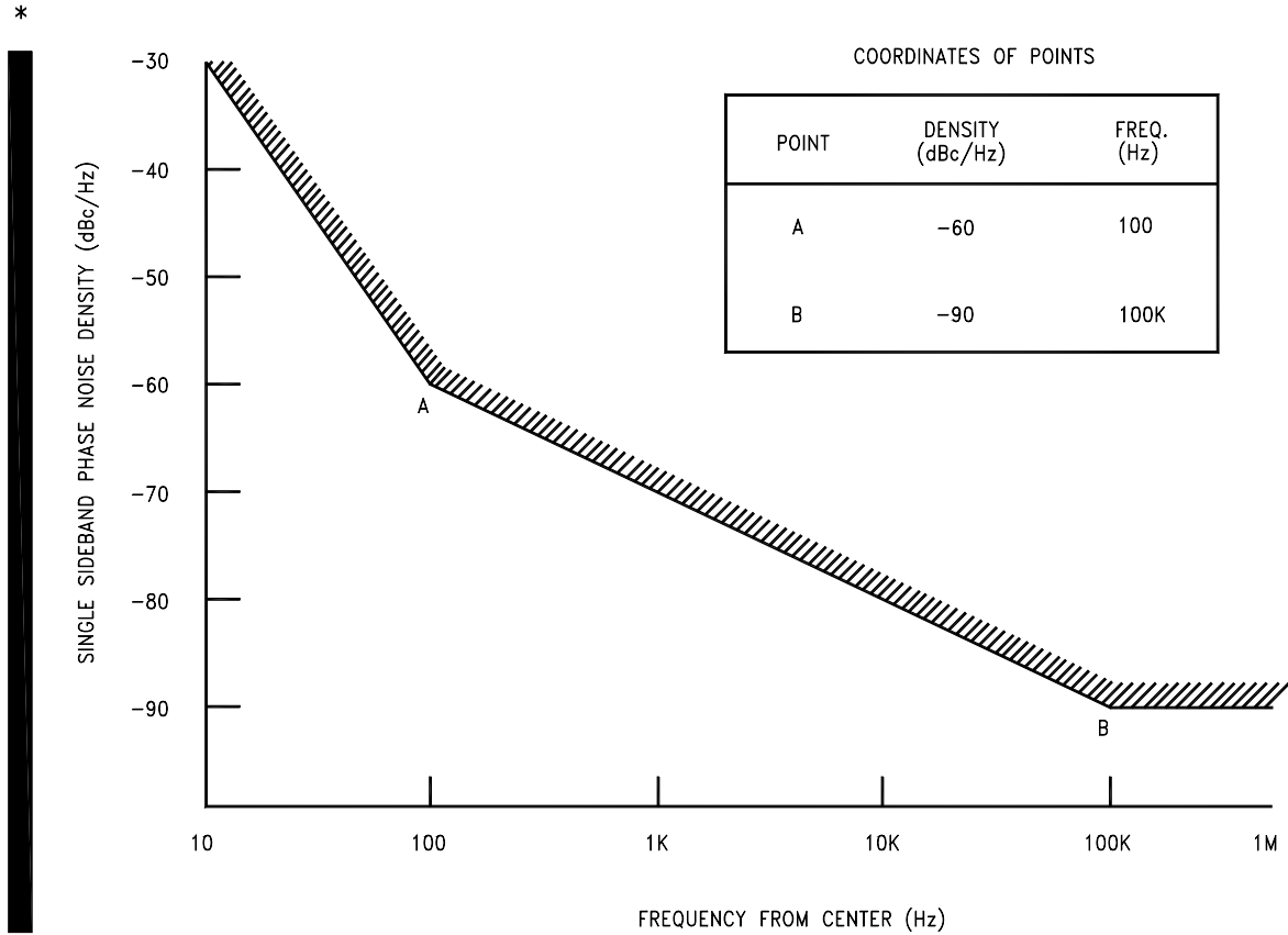
Figure 6 CONTINUOUS SINGLE SIDEBAND PHASE NOISE REQUIREMENT (For Carriers With Information Rates Less Than Or Equal To 2.048 Mbit/s)
