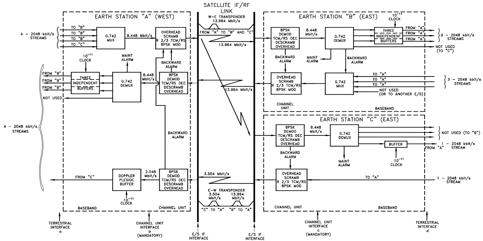
Figure 22 ILLUSTRATION OF MULTI-DESTINATIONAL TCM/IBS APPLICATION (Primary and Secondary Order Carriers)
