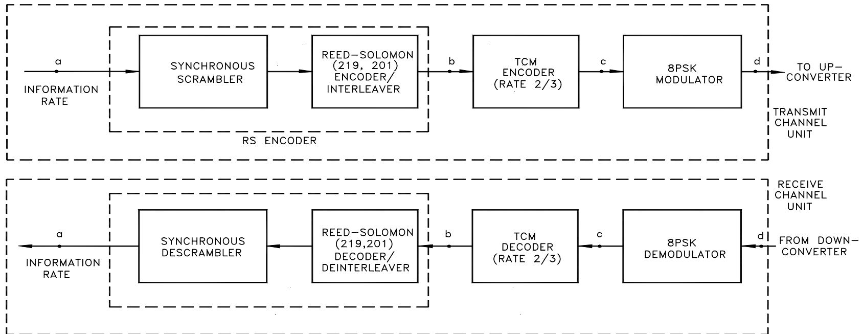
Figure 1 ILLUSTRATION OF TCM/IBS CHANNEL UNIT (Small TCM/IBS Carriers < 1.544 Mbit/s, No Overhead Framing)
