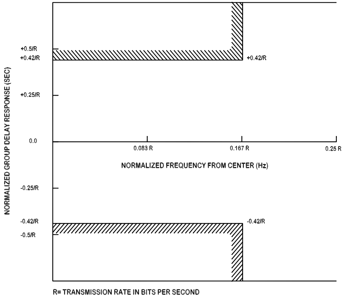
Figure 9 MODULATOR AND DEMODULATOR FILTER GROUP DELAY RESPONSE
