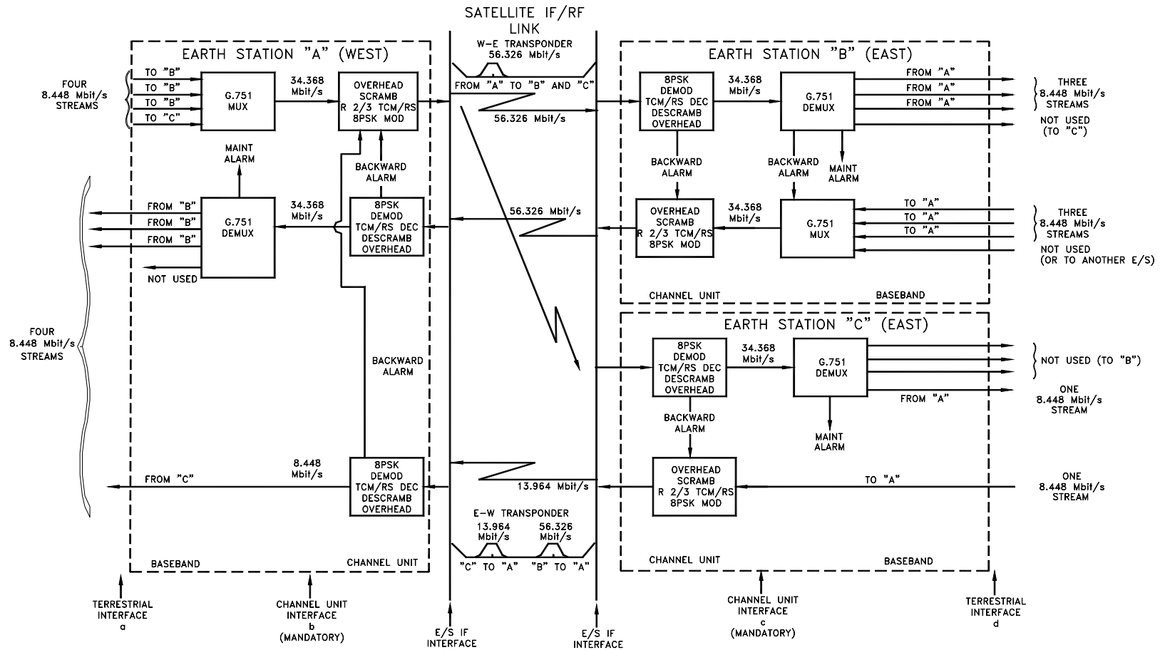
Figure 23 ILLUSTRATION OF MULTI-DESTINATIONAL TCM/IBS APPLICATION (Second and Third Order Carriers)
