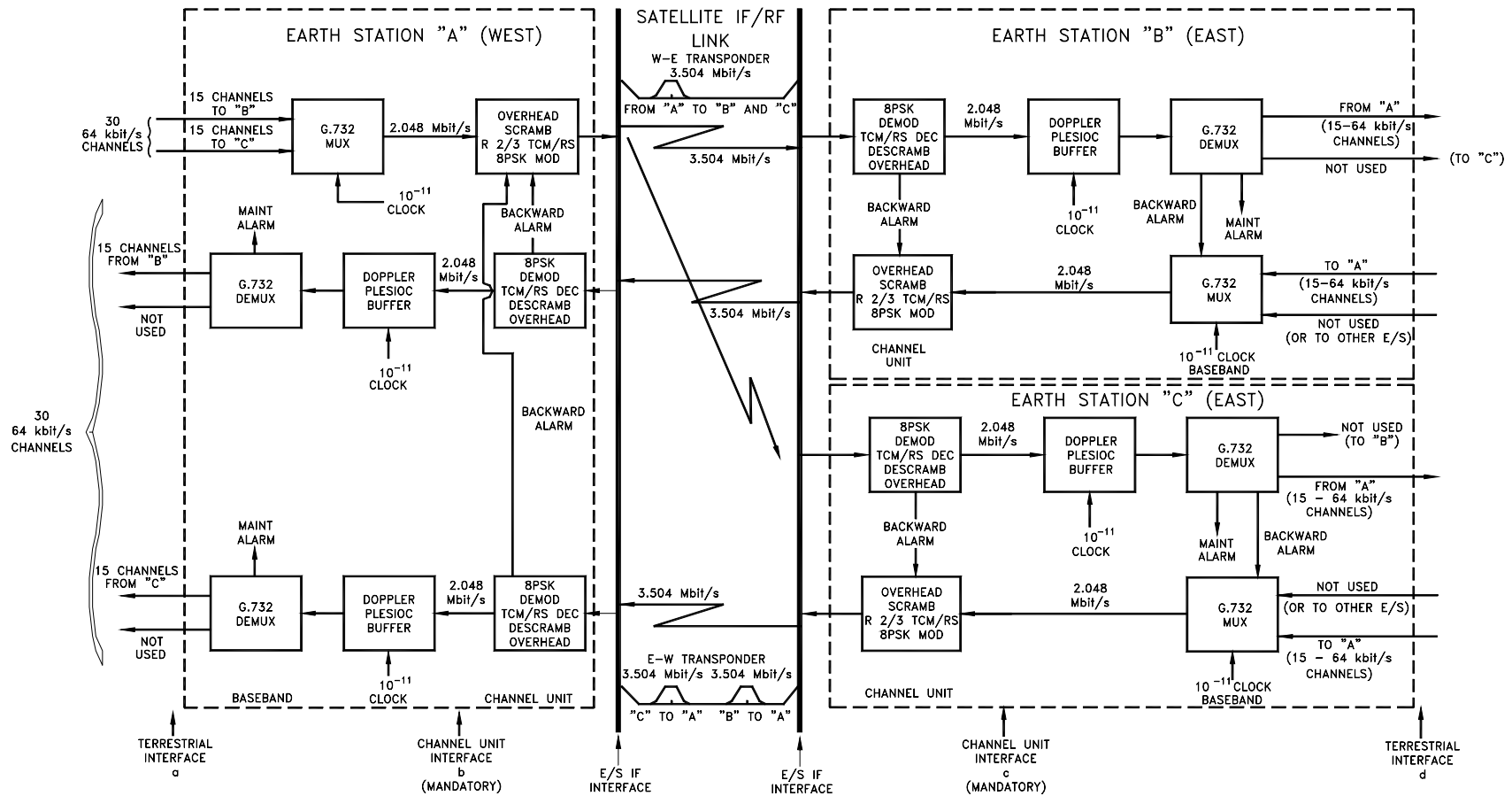
Figure 21 ILLUSTRATION OF MULTI-DESTINATIONAL TCM/IBS APPLICATION (Primary Order Carriers)
