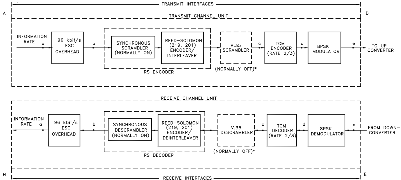
Figure 3 ILLUSTRATION OF TCM/IBS CHANNEL UNIT (TCM/IBS Carriers \geq 1.544 Mbit/s, With Optional 96 kbit/s ESC Overhead Framing)
