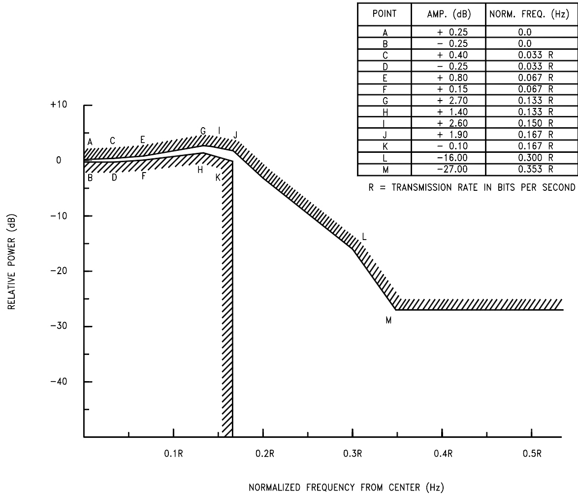
Figure 7 MODULATOR FILTER AMPLITUDE RESPONSE
