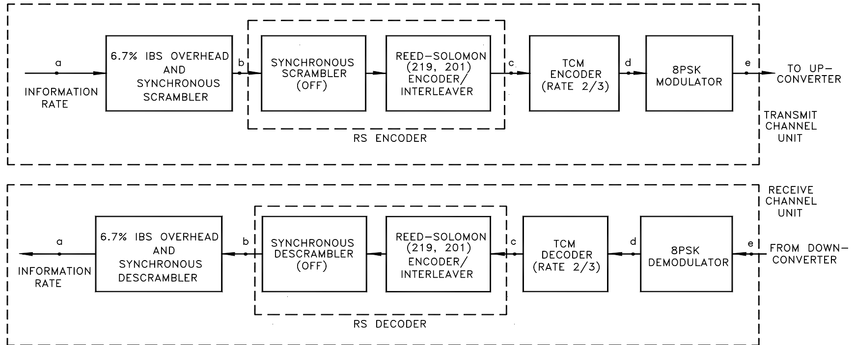
Figure 2 ILLUSTRATION OF TCM/IBS CHANNEL UNIT (Small TCM/IBS Carriers < 1.544 Mbit/s, With IBS Overhead Framing)
