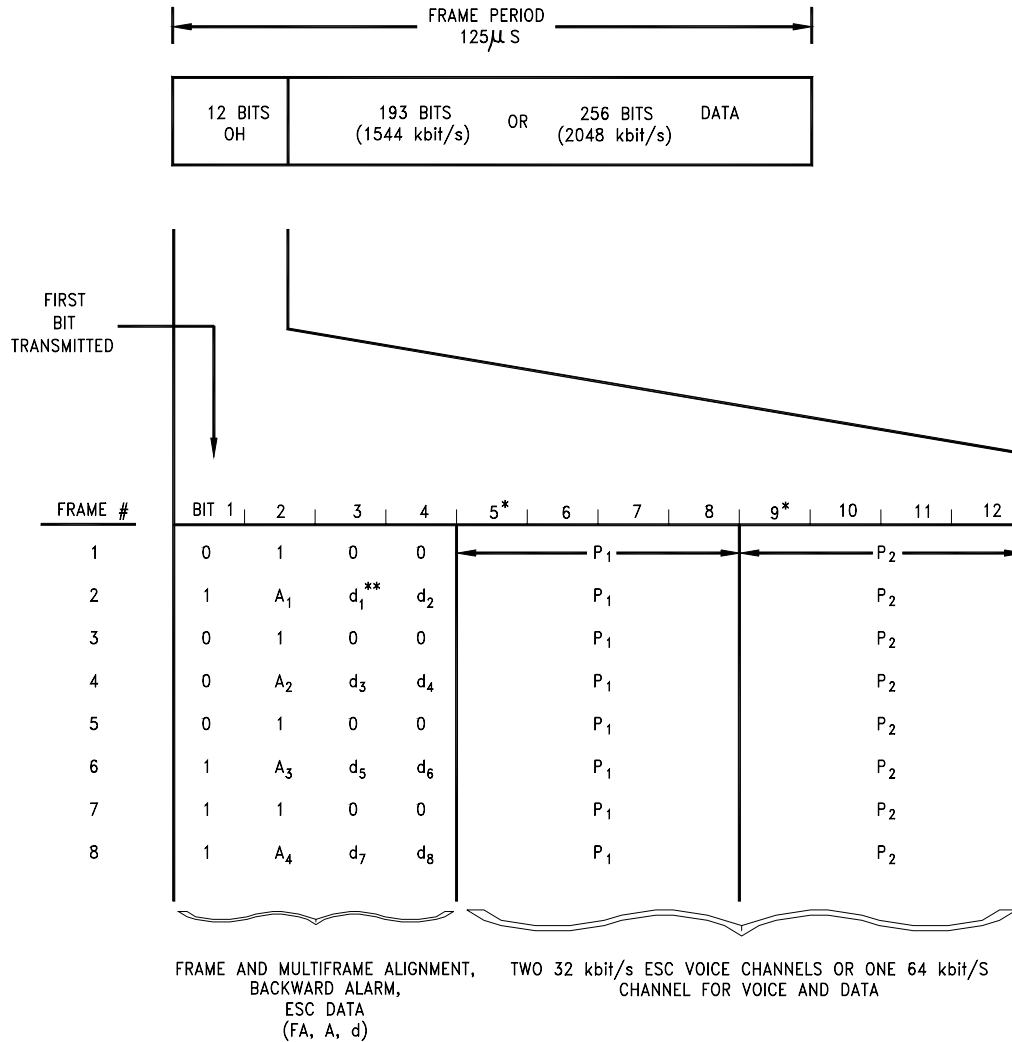
Figure 12 OVERHEAD STRUCTURE FOR 1544 AND 2048 kbit/s TCM/IBS CARRIERS
