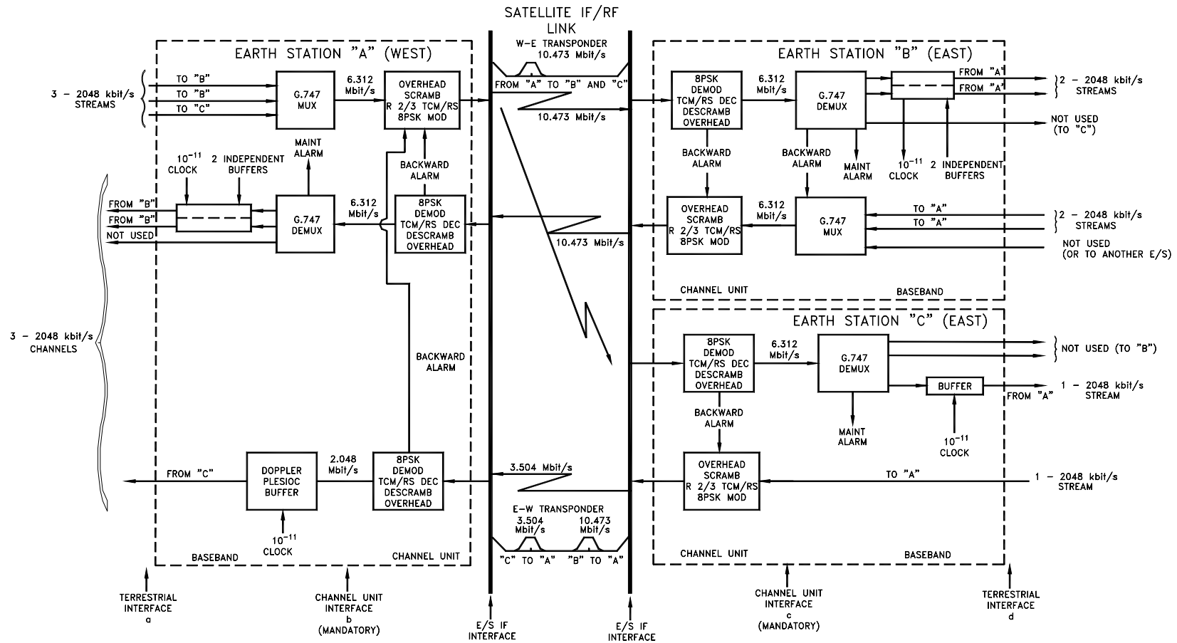
Figure 24 ILLUSTRATION OF MULTI-DESTINATIONAL TCM/IBS APPLICATION (Primary and Second Order Carriers Using the Interworking Hierarchy Bit Rates)
