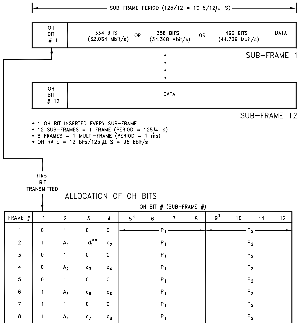
Figure 15 OVERHEAD STRUCTURE FOR 32.064, 34.368 and 44.736 Mbit/s TCM/IBS CARRIERS
